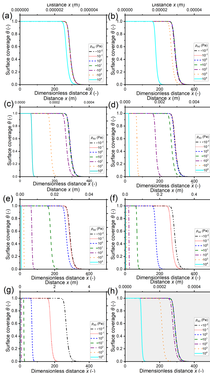
Fig. 7 Saturation profiles in wide lateral high-aspect-ratio channels of various heights at a constant reactant exposure of 10 Pa s (300 °C). Channel heights: (a) 10 nm, (b) 100 nm, (c) 1 μm, (d) 10 μm, (e) 100 μm, (f) 1 mm, (g) 1 cm, and (h) 500 nm (the typical PillarHall™ case 17,37 ). The calculated Knudsen number values for the simulated points are shown in Fig. 3(a). To maintain a constant exposure of 10 Pa s, the pulse time was varied in the range of 10^{-3} to 10^3 s and the initial reactant partial pressure p_{A0} was varied in the range of 10^{-2} to 10^4 Pa (Section S2 in the ESI†). The other simulation conditions are listed in Table 1.
