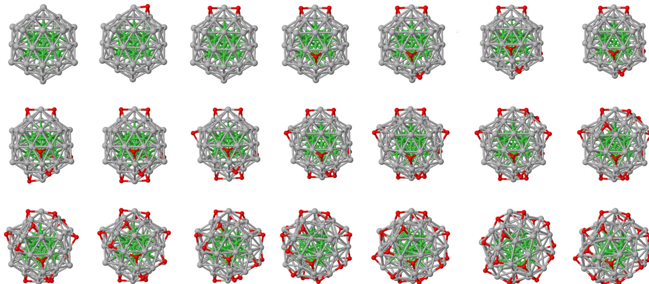
Fig. 1 Putative ground state atomic configurations of \text{Ni}_{13}@Ag_{42}O_m with m = 1 to 20.
