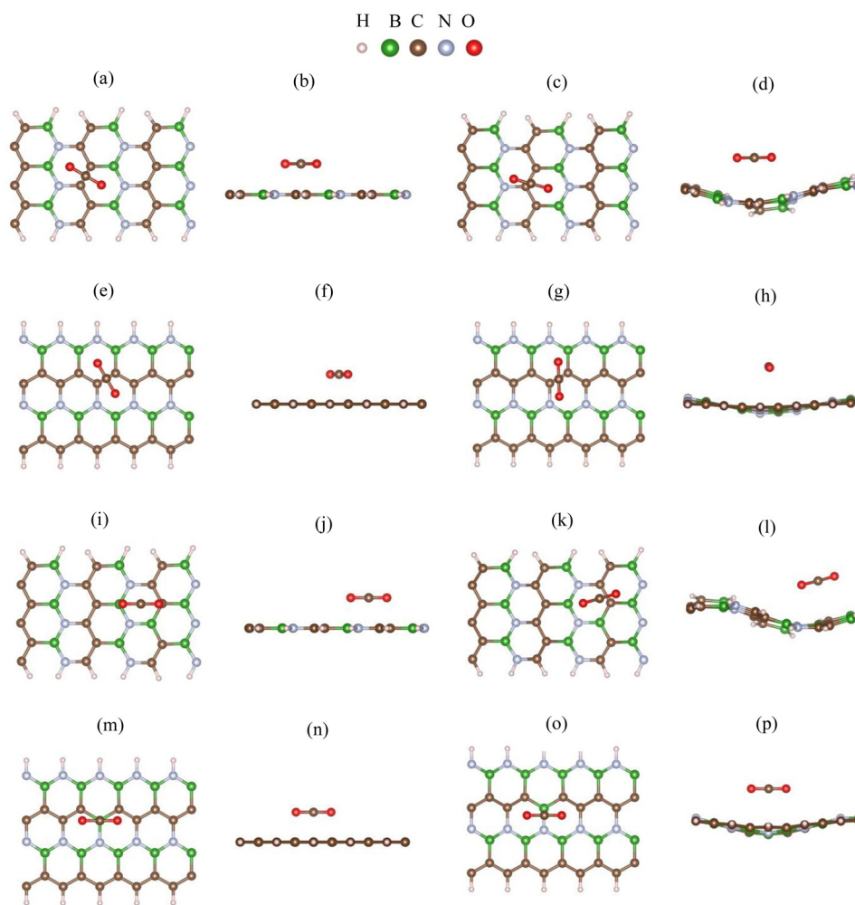
Fig. 8 Top view and side view of the geometric configurations of CO 2 molecule on 6-ABCNNR with 50%-C before (a) and (b) and after (c) and (d) optimization, 8-ZCBNNR with 50%-C before (e) and (f) and after (g) and (h) optimization, B-rich 6-ABCNNR with 50%-C before (i) and (j) and after (k) and (l) optimization, B-rich 8-ZCBNNR with 50%-C before (m) and (n) and after (o) and (p) optimization.
