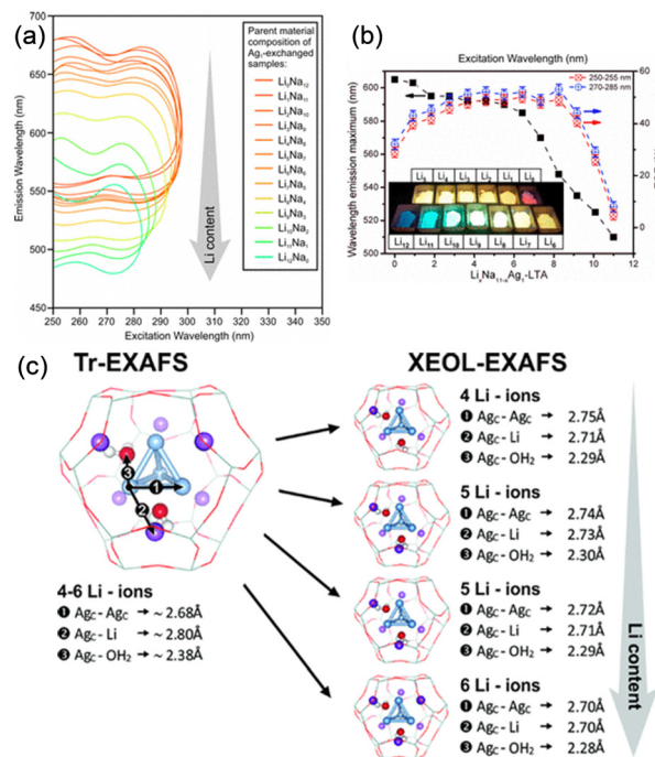
Fig. 6 (a) 2D emission and excitation profiles of the different hydrated Ag-exchanged LTA. (b) Maximal emission wavelength (excitation at 270–285 nm) and external quantum efficiency of the \text{Ag}_1\text{Li}_x\text{Na}_{(1-x)} -LTA depending on the Li content. (c) Schematic representation of the changes observed for the ground and excited states of the tetrahedral Ag clusters as determined by Tr- and XEOL-EXAFS, respectively. Reprinted with permission from Baekelant et al. Copyright 2018 American Chemical Society.
