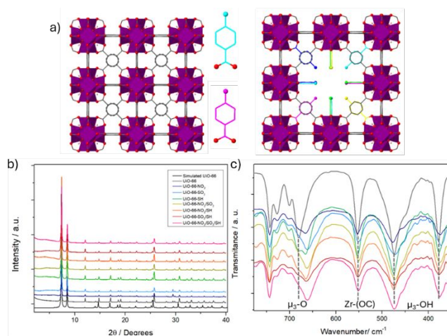
Fig. 1: a) Schematic representation of MTVM MOF with defect-induced reO topology in comparison with the pristine MOF. b) PXRD profiles c) amplification of FT-IR profiles highlighting \mu_3 -O, \mu_3 -OH and Zr-(OC) bands.
