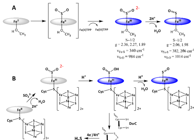
Scheme 1 (A) Mechanism of \text{SO}_2 reduction observed for \text{Fe(II)TPP} . Spectroscopic parameters are indicated below the proposed structures of the intermediates. (B) Mechanism of the SiR is refined based on the mechanism of \text{SO}_2 reduction observed for \text{Fe(II)TPP} . The porphyrin ligand is indicated as a blue circle for clarity.
