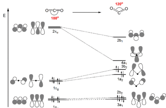
Scheme 4 Qualitative Walsh diagram for the OCO angle bending from 180° to 120°. Most important frontier molecular orbitals of CO 2 are depicted.
