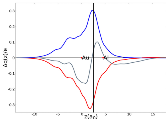
Fig. 9 CD-NOCV curves associated to the first two NOCV deformation densities ( \Delta\rho'_{1\alpha} , in red and \Delta\rho'_{1\beta} , in blue) for the analysis of the Au–Al bond in the [\text{tBu}_3\text{PAuAl}(\text{NON})] complex. The grey curve is associated to the overall deformation density \Delta\rho' . The red dots indicate the position of the nuclei along the z axis. The vertical solid line marks the isodensity boundary between the fragments. Positive (negative) values of the curve indicate right-to-left (left-to-right) charge transfer. Adapted and reprinted with permission from ref. 30 Copyright 2021, American Chemical Society.
