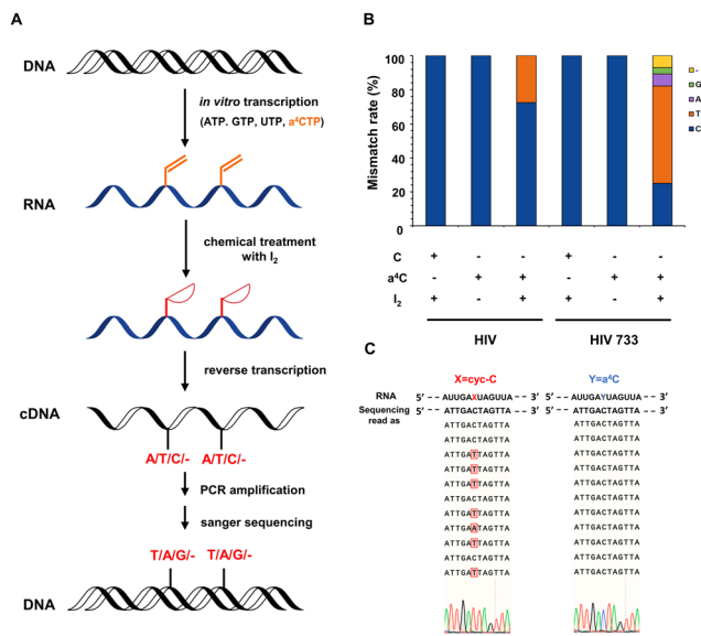
Fig. 2 Chemical sequencing assay to pinpoint a C labelling site on RNA. (A) Schematic illustration of identifying the a C site on the in vitro transcribed RNA. a C can be incorporated into the RNA probe through in vitro transcription, and iodination of a C leads to the formation of cyc-C, which induces base mismatch in the synthesis of complementary DNA (cDNA) during RT. (B) Base mismatch rates of a C and cyc-C in the presence of commercial HIV recombinant reverse transcriptase (HIV) or its mutant HIV 733. (C) The selected Sanger sequencing results of amplified cDNAs using HIV 733.
