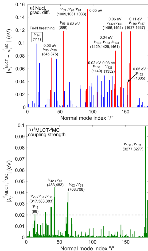
Fig. 6 Analysis of vibronic effects for the lowest four 3 MLCT and three 3 MC states of [Fe(bmip) 2 ] 2+ at the FC geometry. (a) Largest absolute difference of nuclear gradients ( |k_i^{3MLCT} - k_i^{3MC}| ) for all normal modes. For each mode, the 3 MLCT- 3 MC component leading to the largest absolute difference is selected. Absolute differences above 0.02 eV originating from a significant k_i^{3MLCT} > 0.02 eV value are highlighted in red. The numbers in eV next to mode labels are the absolute values of the largest 3 MLCT gradient components. (b) 3 MLCT- 3 MC coupling strengths ( |\lambda_i^{3MLCT, 3MC}| ) for all normal modes. For each mode, the 3 MLCT- 3 MC component leading to the largest coupling strength is selected. In parentheses, the frequency of the most important modes is given (in cm -1 , for both panels).
