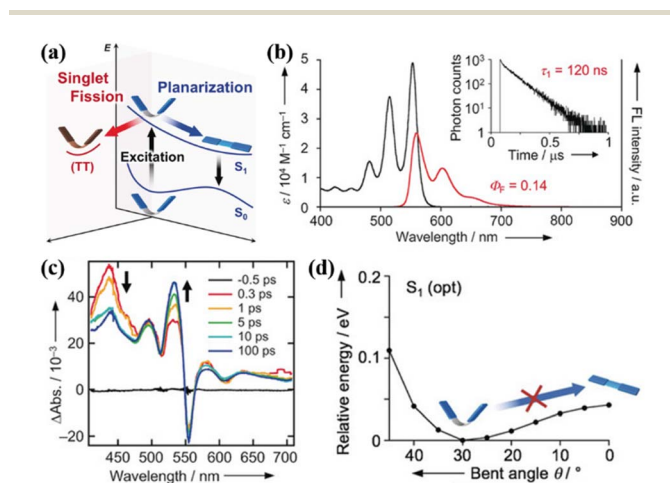
Fig. 12 (a) Energy diagram of the COT-fused dimers. Two possible dynamics, conformational planarization in S_1 and SF to a correlated triplet pair ^1(\text{TT}) , are indicated. (b) UV/vis absorption (black) and FL (red) spectra of dimer 39. Fluorescence quantum yield ( \phi_f ) is considered in the area of the fluorescence spectra. The fluorescence decay curve of dimer 39 is shown in the inset of (b). (c) TA spectra of dimer 39 in \text{CH}_2\text{Cl}_2 . (d) S_1 energy profiles with respect to conformational planarization of dimer 39. Reproduced with permission. 163 Copyright 2018, Wiley-VCH.
