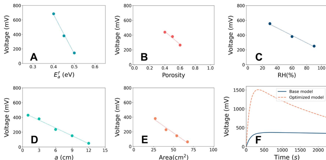
Fig. 4 Parametric effect on the output voltage from (A.) catalytic activation barrier for the forward reaction, (B.) porosity, (C.) relative humidity at the right half of substrate (RH), (D.) length of the side adjacent to a water droplet (denoted as a ), and (E.) total area of CB film. (F.) Time course of output voltage according to the base model and optimized model.
