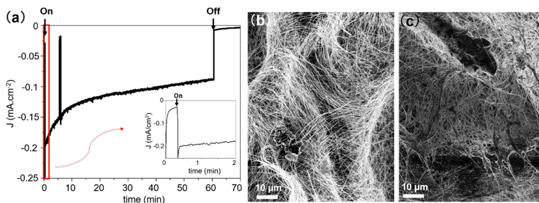
Fig. 7 (a) Chronoamperometry of PCS-SiNW-MoS x at -0.15 V vs. RHE in 0.5 M H 2 SO 4 under illumination (48 nm-SiNWs, Δ Q MoS x = 6 mC cm -2 ) with N 2 bubbling. SEM images of the electrode before (b) and after (c) the stability test.
