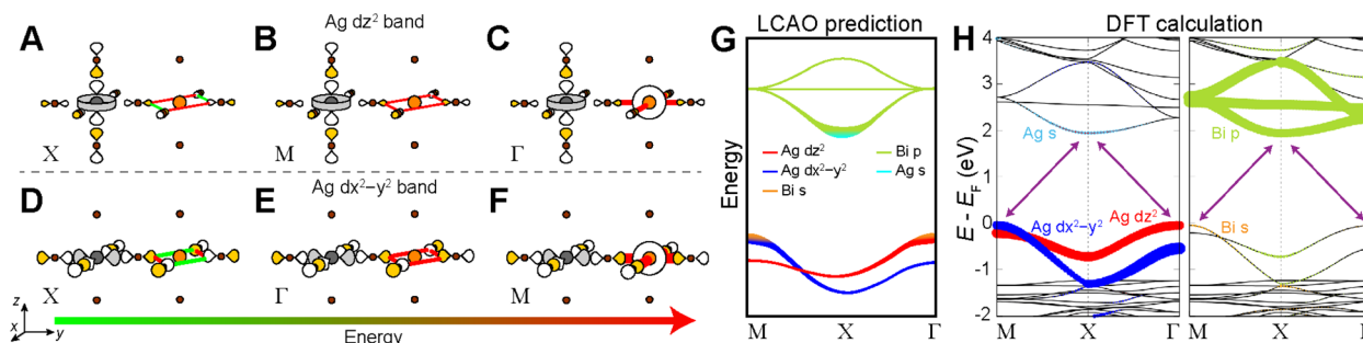
Fig. 8 LCAO analysis for the n = 1 Ag–Bi structure. LCAO representations of the Ag d_{z^2} derived valence band (VB) at the \text{X} (A), \text{M} (B), and \Gamma (C) points ranked in order of increasing energy from left to right. LCAO representations of the Ag d_{x^2-y^2} derived VB at the \text{X} (D), \Gamma (E), and \text{M} (F) points ranked in order of increasing energy from left to right. Bonding and antibonding interactions at the \text{B}' site are shown as green and red lines, respectively, and the thickness of each line corresponds to the strength of the interaction. Halide p orbital lobes are scaled to represent approximate relative electron densities and the shading of orbital lobes denote their relative phases. Gray, orange, and brown spheres represent Ag, Bi, and Br atoms, respectively. (G) Predicted band diagram of the n = 1 Ag–Bi structure using our LCAO analysis. (H) DFT band structure of the n = 1 Ag–Bi structure without SOC. The band structure is shown in duplicate where the Ag (left panel) and Bi (right panel) states that compose the bands are represented by colored dots.
