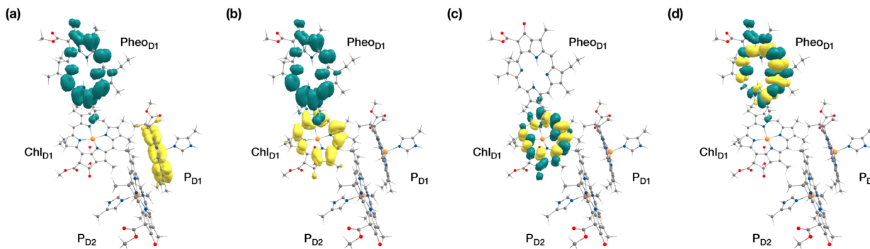
Fig. 5 Difference density densities describing the lowest singlet-triplet excitations of the D1 branch in PSII: (a) the lowest triplet excitation with {}^3[\text{P}_{\text{D1}}^{\delta+}\text{PheO}_{\text{D1}}^{\delta-}] charge transfer character; (b) the lowest triplet excitation with {}^3[\text{Chl}_{\text{D1}}^{\delta+}\text{PheO}_{\text{D1}}^{\delta-}] charge transfer character; (c) local {}^3\text{Chl}_{\text{D1}} excitation; (d) local {}^3\text{PheO}_{\text{D1}} excitation.
