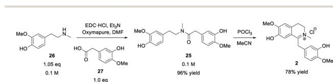
Scheme 4 Protecting group-free amide coupling of building block 26 with acetic acid derivative 27 followed by a Bischler–Napieralski-type cyclization of amide 25 towards iminium ion 2 .
