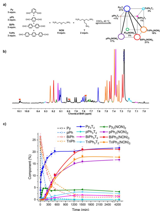
Fig. 10 (a) [4 \times 2] square prismatic DC_{ov}L generated from 3Py + 3pPh + 3BiPh + 3TriPh + 3T + 9NON ; (b) partial ^1H NMR spectrum (400 MHz, CDCl_3 , 40 ^{\circ}C ) of the equilibrated reaction mixture; (c) ^1H NMR monitoring of macrocycles and macrocyclic cages over 4260 min. The initial concentration of each dialdehyde was 2.0 mM. The signals of free dialdehydes BiPh and TriPh are indicated by red and orange stars, respectively. The larger size and the bold diagonal lines indicate the selective cogeneration of agonistic constituents. The spectra and kinetic curves are coloured in accordance with the molecular structures.
