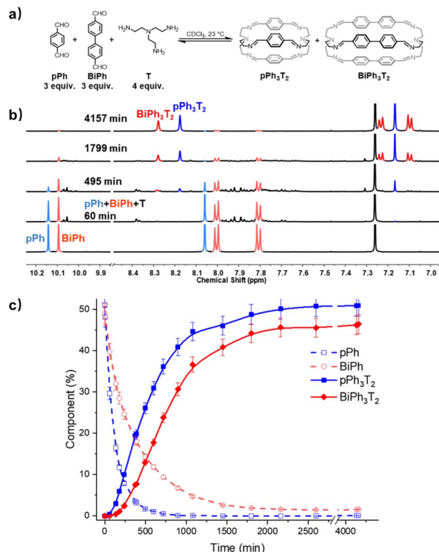
Fig. 5 (a) Component self-sorting in the competitive formation of two macrobicyclic cages p Ph 3 T 2 , BiPh 3 T 2 . (b) Evolution of the partial 1 H NMR spectra (500 MHz, CDCl 3 , 23 °C) of the reaction 3 p Ph + 3BiPh + 4T ([ p Ph] 0 = [BiPh] 0 = 3.6 mM, [T] 0 = 4.8 mM) over 4157 min. The bottom trace corresponds to the dialdehyde components, p Ph and BiPh. (c) 1 H NMR monitoring of dialdehydes p Ph, BiPh and cages p Ph 3 T 2 , BiPh 3 T 2 over 4157 min. The distribution (%) have been obtained by the integration of the aromatic regions and aldehyde CHO proton signals in the 500 MHz 1 H NMR spectra. Error in 1 H-NMR signal integration: ±5%. The corresponding t 1/2 values are given in the ESI.†
