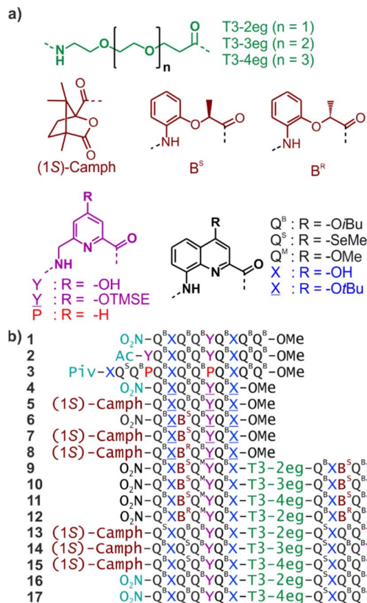
Fig. 1 (a) Structures of di-, tri- and tetraethylene glycol T3 spacers, chiral (1S)-camph, B^S and B^R units, and Q , X , P and Y amino acid monomers. Q^B carries organic solubilizing side chains. Q^S was introduced in some sequences to assist crystallographic structure elucidation using the anomalous scattering of Se, though it turned out to be unneeded. Q^M is isosteric to Q^S . X and Y are the protected precursors of hydrogen-bonding monomers X and Y , respectively. TMSE = 2-trimethylsilylethyl. (b) Oligoamide foldamer sequences. Piv = pivaloyl. In sequences ending with an 8-nitro group, this group replaces the terminal amine.
