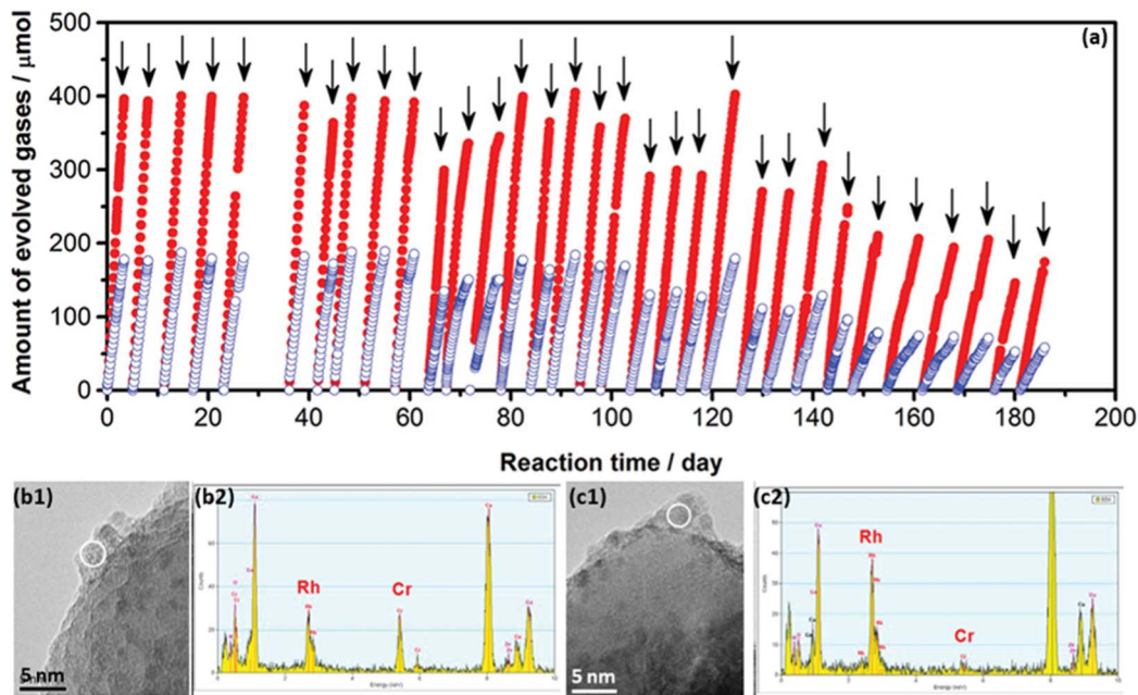
Fig. 4 (a) Long-term measurement of Rh 2-y Cr y O 3 /GaN:ZnO photocatalyst for overall water splitting under visible light. (b and c) Combination of TEM and EDS analysis for the Rh 2-y Cr y O 3 /GaN photocatalyst (b) before and (c) after deactivation. Reproduced from ref. 51, copyright 2012, American Chemical Society.
