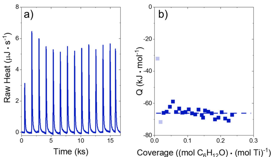
Fig. 9 (a) Thermogram from the titration of Ti-BEA-OH with 1,2-epoxyhexane (10 mM \text{C}_6\text{H}_{12}\text{O} in x_{\text{C}_4\text{H}_6\text{O}_2} = 0.25 (7.6 M), 313 K, 1 \mu\text{L} per injection) during isothermal titration calorimetry (ITC), and (b) the corresponding heats released as a function of 1,2-epoxyhexane coverage. Transparent points are omitted due to common errors associated with early injections.
