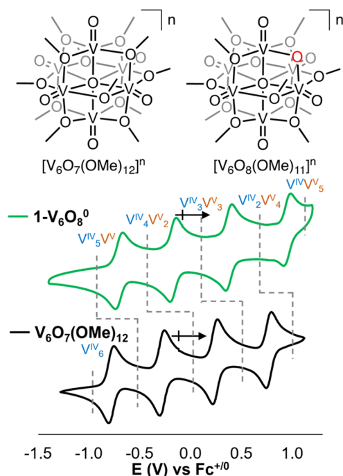
Fig. 1 CV of 1 mM 1-V 6 O 8 0 (green, top) and V_6O_7(OMe)_{12} (black, bottom) in MeCN with 100 mM [^nBu_4N][PF_6] supporting electrolyte (scan rate = 100 mV s -1 ). Labelled on the curves are the structures, oxidation state distributions for each charge state of the cluster, and the open circuit voltages indicated with a black arrow.
