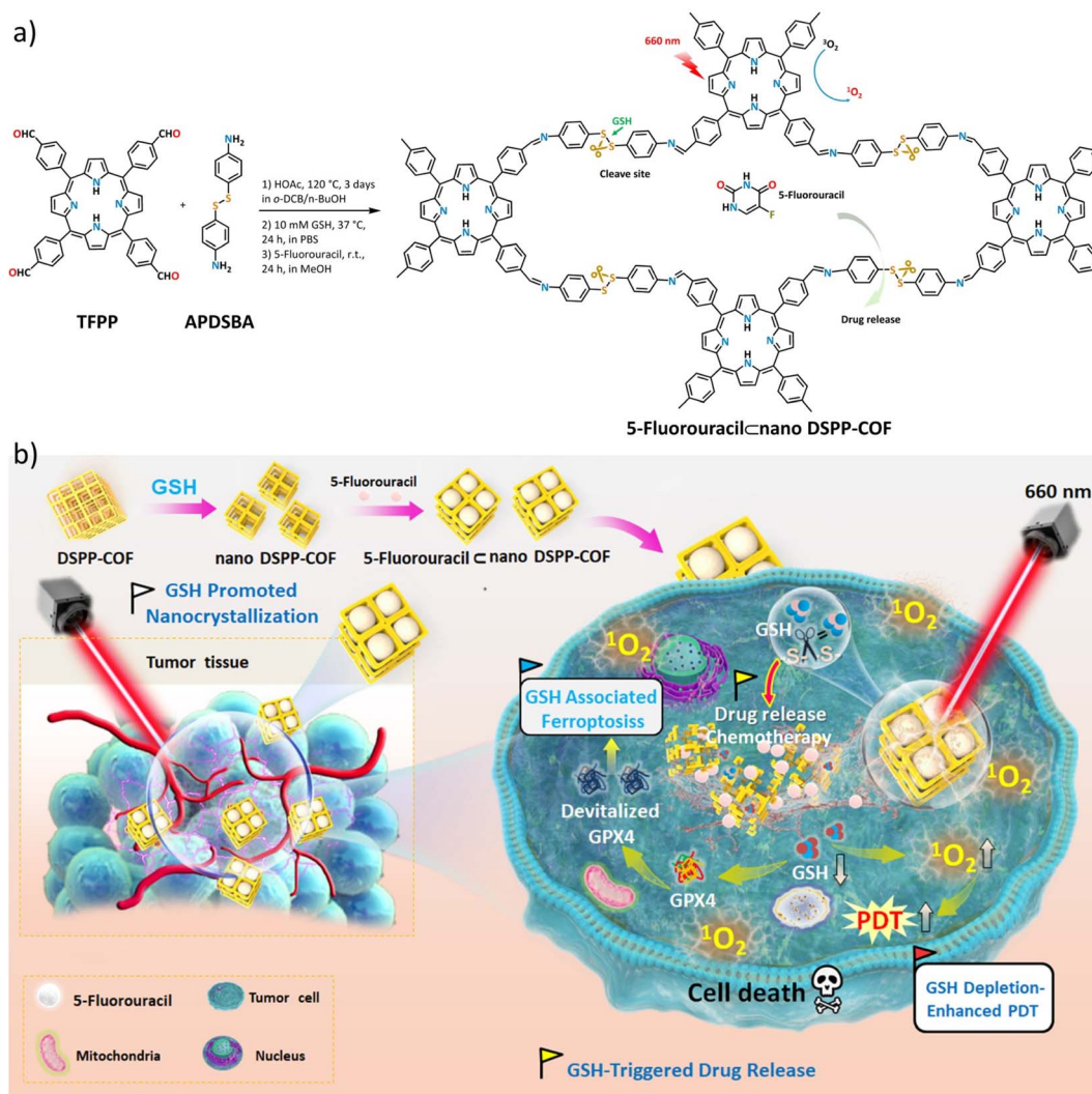
Scheme 1 (a) Synthesis of DSPP-COF, nano DSPP-COF, and 5-Fu \subset nano DSPP-COF. (b) Synthesis and treatment application of 5-Fu \subset nano DSPP-COF, including GSH-promoted DSPP-COF nanocrystallization, 5-Fu loading, and the obtained 5-Fu \subset nano DSPP-COF for combination antitumor treatment by endogenous GSH-triggered drug release and GSH depletion-enhanced PDT via the ferroptosis pathway.
