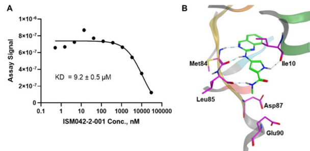
Fig. 6 (A) Representative binding affinity curve of ISM042-2-001 in CDK20 kinase binding assay. Data points are presented as the mean of three independent wells in one experiment. Similar results were obtained in three independent experiments and the KD is the mean \pm SD of three independent experiments. (B) Predicted binding pose for ISM042-2-001 with CDK20.
