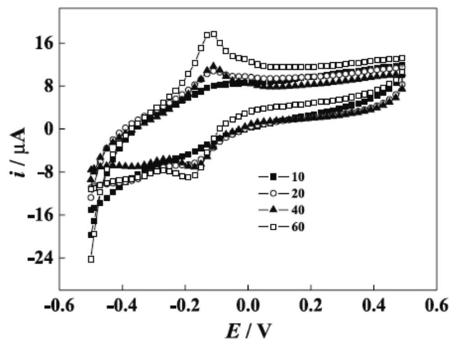
Fig. 7 Voltammogram of poly(safranin) generated at different cycles (10, 20, 40, and 60 cycles) in 0.1 M sulfuric acid solution. This figure has been adapted/reproduced from ref. 6 with permission from PubliSBQ, copyright (2023).
