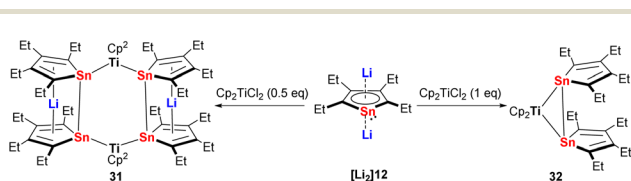
Scheme 5 Reaction of tetraethyldilithiostannole [\text{Li}_2]\textbf{12} with [\text{Cp}_2\text{TiCl}_2] , leading to the formation of 31 and 32 . 33
