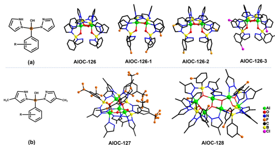
Fig. 1 A display of all compounds isolated herein showing the association of structure type and ligand regulation. (a) The alternation of functional groups on the benzene ring results in the AIOc-126 series. (b) The change on both the benzene ring and pyrazole brings the nuclearity increment, see compounds AIOc-127 and AIOc-128 .
