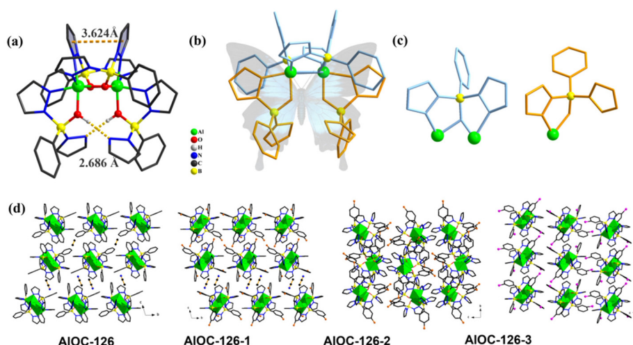
Fig. 2 The molecular structures of the dimers of AIOc-126 series. (a) Molecular structures of AIOc-126 and coordination environment of Al(III). (b) Simplified structure of AIOc-126 . (c) Coordination mode of [Ph(pz)B(μ-O)(pz)]. (d) Lattice arrangements of AIOc-126 series (color code: Al green; B yellow; O red; N blue; C black).
