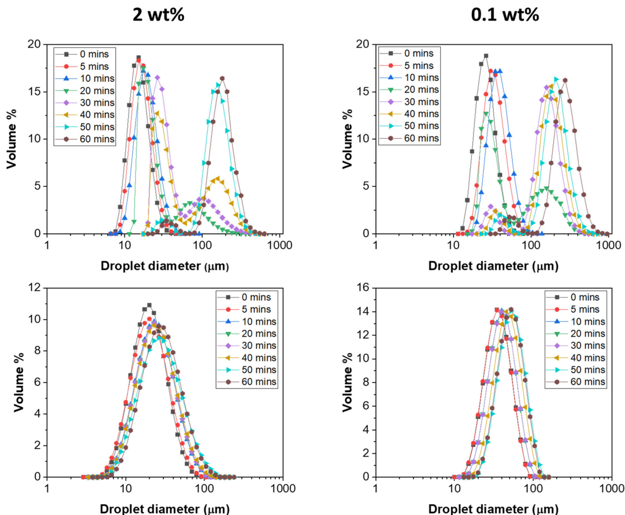
Fig. 1 Evolution of the droplet size and size distribution of n -dodecane in water emulsions produced using an Ultra-Turrax homogeniser operated at 12 000 rpm for 2 minutes over time, measured by laser diffraction. These emulsions were designed with a dispersed phase volume of 10% and stabilised by 88% hydrolysed PVA at 2 different molecular weights (LMw-PVA-88 and HMw-PVA-88) and at two different polymer concentrations (0.1 and 2 wt%).
