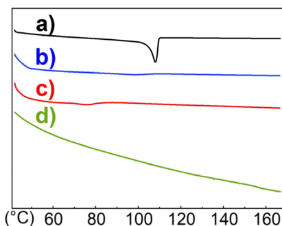
Fig. 3 DSC curves (left) and photographs (middle and right) of the representative polyethylene samples with diverse microstructures: (a) (Table 1, entry 2), (b) (Table 1, entry 24), (c) (Table 1, entry 4) and (d) (Table 1, entry 16).
