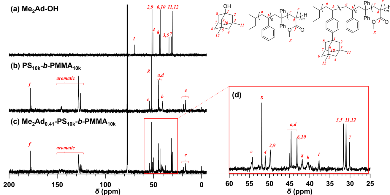
Fig. 3 ^{13}\text{C} NMR spectra of (a) \text{Me}_2\text{Ad-OH} and (b) \text{PS}_{10\text{k}}\text{-b-PMMA}_{10\text{k}} in \text{CDCl}_3 (100 MHz), and (c) inverse-gated decoupling ^{13}\text{C} NMR spectrum of \text{Me}_2\text{Ad}_{0.41}\text{-PS}_{10\text{k}}\text{-b-PMMA}_{10\text{k}} (lower) in \text{CDCl}_3 (100 MHz). (d) The expansion from 60 to 25 ppm of the spectrum (c).
