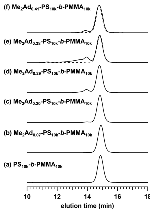
Fig. 5 SEC traces of \text{Me}_2\text{Ad-PS}_{10\text{k}}\text{-b-PMMA}_{10\text{k}} samples (b)-(f) and the corresponding \text{PS}_{10\text{k}}\text{-b-PMMA}_{10\text{k}} (a) (eluent, THF; flow rate, 1.0 \text{ mL min}^{-1} ). The dashed curves represent the SEC traces after preparative SEC purification.
