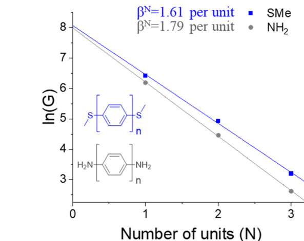
Fig. 6 Plot of the most probable experimental conductance values \ln(G) of \text{MeS}\{(\text{C}_6\text{H}_4)_N\}\text{SMe} and \text{H}_2\text{N}\{(\text{C}_6\text{H}_4)_N\}\text{NH}_2 , 36 versus number of para -phenylene units -\text{C}_6\text{H}_4- , N .
