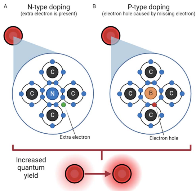
Fig. 2 N-Type doping vs. P-type doping. 33 (A) N-Type doping, reliant on the presence of an extra electron in the carbon dot structure. (B) P-Type doping, where an electron hole acts as a positive particle.
