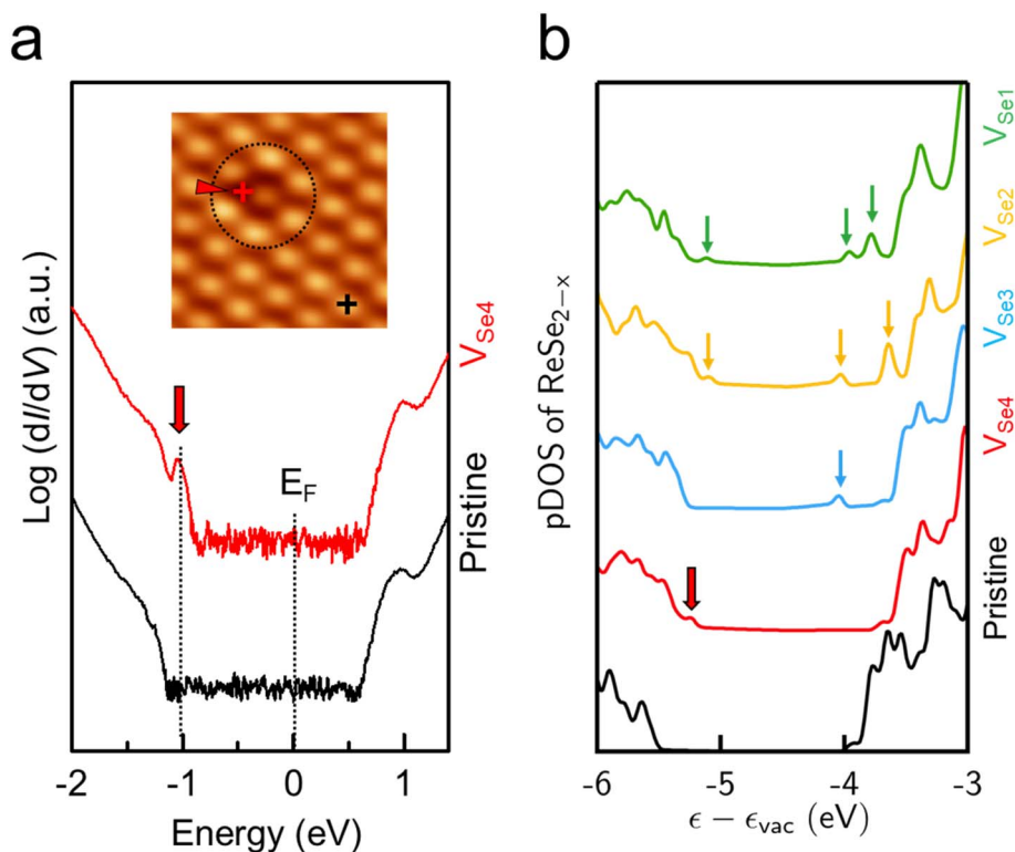
Fig. 3 The defect state of the Se 4 vacancy. (a) dI/dV spectra were measured at the Se 4 defect site (red curve) and defect-free area (black curve). The inset shows an STM image where STS measurements were taken (color coded). The Se 4 vacancy is indicated by the red triangle. (b) The partial density of states (pDOS) was calculated based on the DFT HSE06 functional for different upper Se vacancies and pristine ReSe 2-x ; the green, orange, blue, red, and black curves correspond to the pDOS of Se 1 , Se 2 , Se 3 and Se 4 vacancies and pristine ReSe 2 , respectively.
