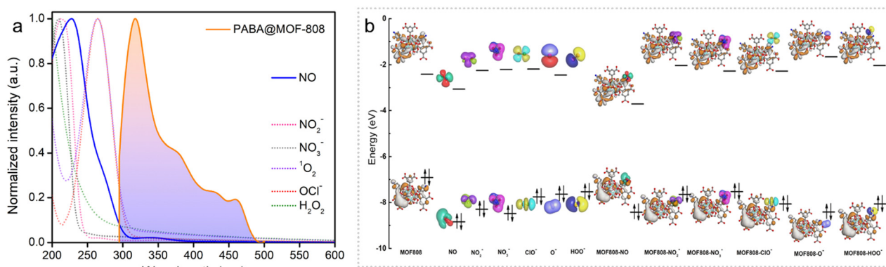
Fig. 3 (a) Spectral overlap between UV-vis spectra of different ROS/RNS and photoluminescence (PL) emission spectra of PABA@MOF-808. (b) HOMO and LUMO energy levels of the PABA@MOF-808 unit and different ROS/RNS along with NO.
