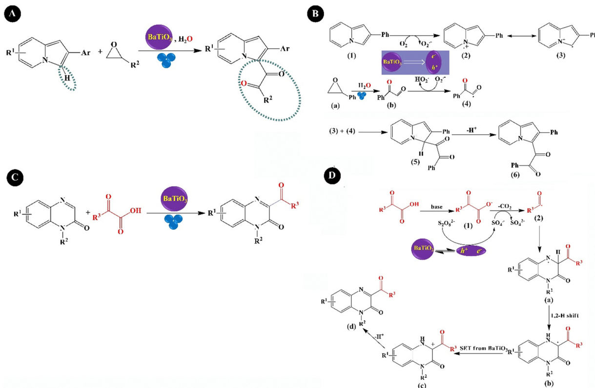
Fig. 11 The mechano-induced synthesis procedure (A) and mechanism (B) of 1,2-diketotoindolizine from indolizines and epoxides over BaTiO 3 (adapted from ref. 211 with permission from American Chemical Society). The mechano-induced synthesis (C) and mechanism (D) of C3-acylation quinoxalin-2(1H)-ones (adapted from ref. 213 with permission from American Chemical Society).
