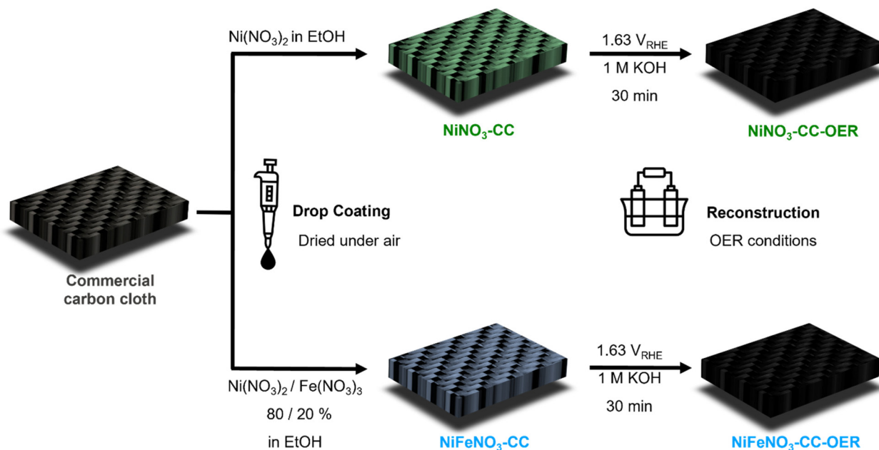
Fig. 1 Schematic illustration of the electrode preparation. Commercial carbon cloth (CC) was activated through acid treatment (HNO 3 ). Ni(NO 3 ) 2 and a mixture of 80% Ni(NO 3 ) 2 and 20% Fe(NO 3 ) 3 was drop coated onto the carbon cloth and the substrate was dried under air. Subsequently, the electrodes were activated at 1.63 V RHE in 1.0 M KOH for 30 minutes to ensure full reconstruction into the respective oxyhydroxides.
