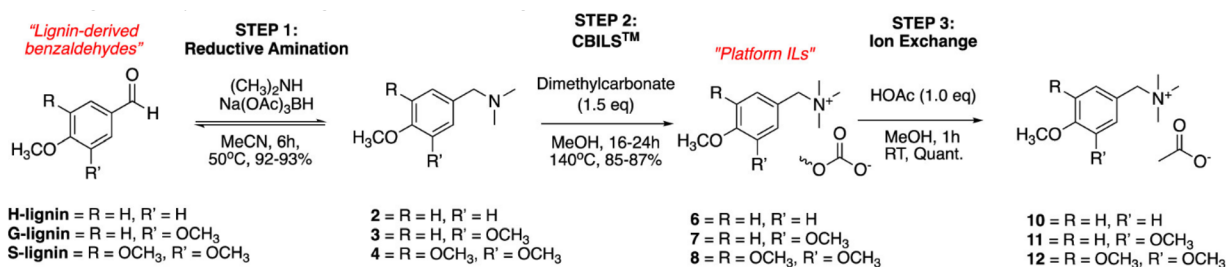
Scheme 20 Three-step synthesis of lignin derived ILs from methylated lignin-derived benzaldehydes. Reproduced with permission from V. Diez, A. DeWeese, R. S. Kalb, D. N. Blaich and A. M. Socha, Ind. Eng. Chem. Res. , 2019, 58 , 16009–16017 (ref. 159). Copyright 2020 American Chemical Society.
