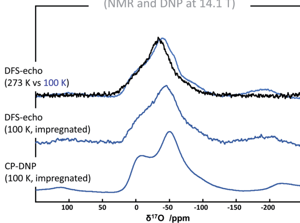
Fig. 4 ^{17}\text{O} MAS NMR spectra of (a) m -CPPT \beta and (b) t -CPPD after ^{17}\text{O} -labelling using BM, recorded at different magnetic fields (9.4, 14.1, 18.8 and 35.2 T). Zoom into the lineshapes recorded at 35.2 T is provided in the ESI (Fig. S3†). (c) Low-temperature ^{17}\text{O} MAS NMR and DNP-enhanced NMR analyses of the m -CPPT \beta phase at 14.1 T (see experimental section for details). “*” symbols correspond to spinning sidebands.
