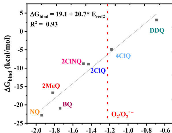
Quinone Second Reduction Potential (V vs. Fc/Fc + )
