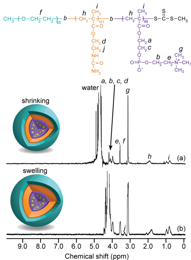
Fig. 4 ^1\text{H} NMR spectra for \text{C}_{70}/\text{EUM} in \text{D}_2\text{O} at (a) 25^\circ\text{C} and (b) 80^\circ\text{C} .
