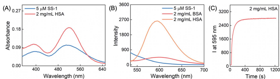
Fig. 1 Optical responses of SS-1 toward HSA. (A) UV-vis absorption changes upon addition of 2 mg mL -1 HSA into a 5 \mu\text{M} SS-1 -containing PBS system. (B) The corresponding changes in the fluorescence spectra. (C) Time-dependent fluorescence intensity change in the reaction system at 595 nm. \lambda_{\text{ex}} = 505 \text{ nm} ; \lambda_{\text{em}} = 525\text{--}700 \text{ nm} ; slit 5/5 nm; 700 V.
