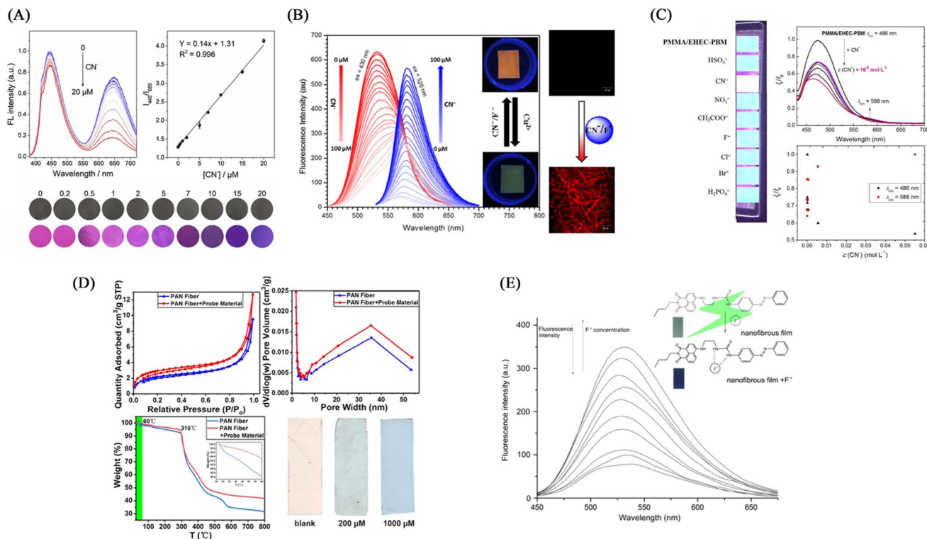
Fig. 20 Sensing properties of \text{CN}^- , \text{F}^- sensor (A) reprinted with permission from ref. 125. Copyright 2019, Elsevier. (B) Reprinted with permission from ref. 126. Copyright 2018, Elsevier. (C) Reprinted with permission from ref. 127. Copyright 2020, Elsevier. (D) Reprinted with permission from ref. 128. Copyright 2022, American Chemical Society. (E) Reprinted with permission from ref. 129. Copyright 2021, Huan Zhang et al.
