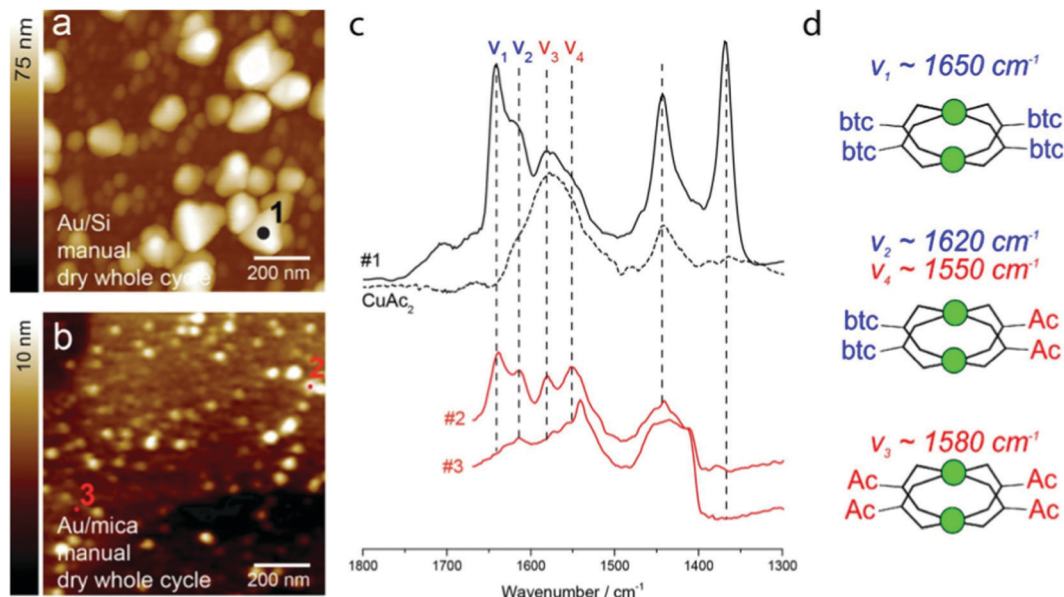
Fig. 4 AFM images and photo-thermal nanoinfrared (AFM-IR) spectra recorded on Au/Si and Au/mica HKUST-1 SURMOF thin films. (a) AFM image of a thin film on Au/Si measured after 5 deposition cycles using manual synthesis with drying each whole cycle. (b) AFM image of a thin film on Au/mica measured after 2 deposition cycles grown in the same way as (a). (c) Representative nano-IR spectra recorded at different positions for the substrates presented in (a), (b). Spectrum (#1) is taken on top of a large SURMOF grain (1 black), spectra #2 and #3 are taken at two different positions. An IRRAS spectrum of CuAc 2 (dotted line) is added for comparison. (d) Vibrational modes assigned to COO@ originating from the different Cu-paddle-wheel substitutions. Note that models are simplified for clarity by omitting C and O atoms coordinated to copper; copper atoms are depicted in green. (Reprinted from Delen et al. 41 ).
