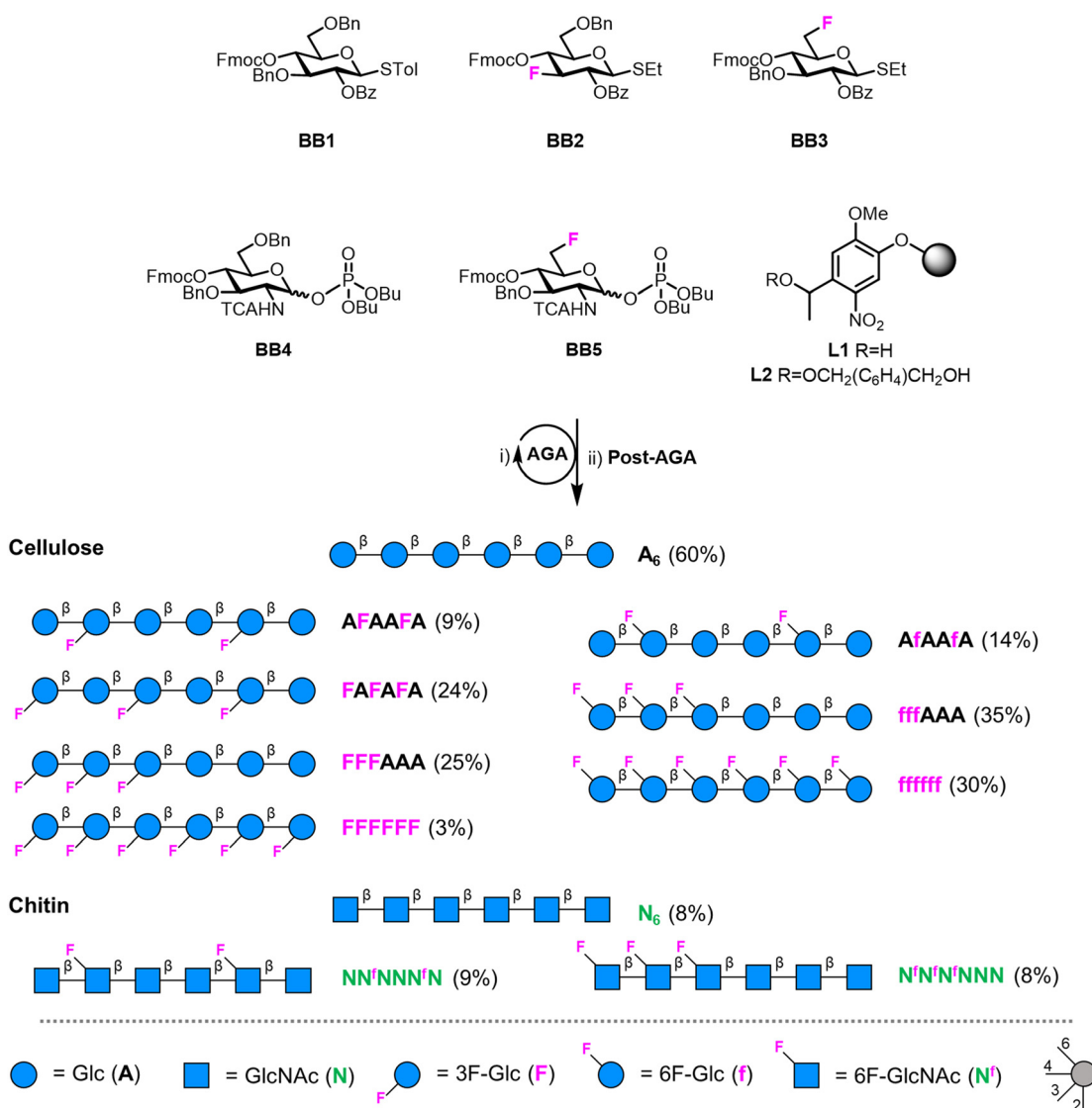
Fig. 4 AGA of fluorinated cellulose and chitin oligomers. Yields of isolated products after AGA, deprotection, and purification are reported in parentheses (see the ESI†). The oligomers A 6 , N 6 , A F A A F A and F A F A F A were synthesized according to previously reported protocols. 22 The oligosaccharides are represented following the Symbol Nomenclature For Glycans (SNFG). 56
