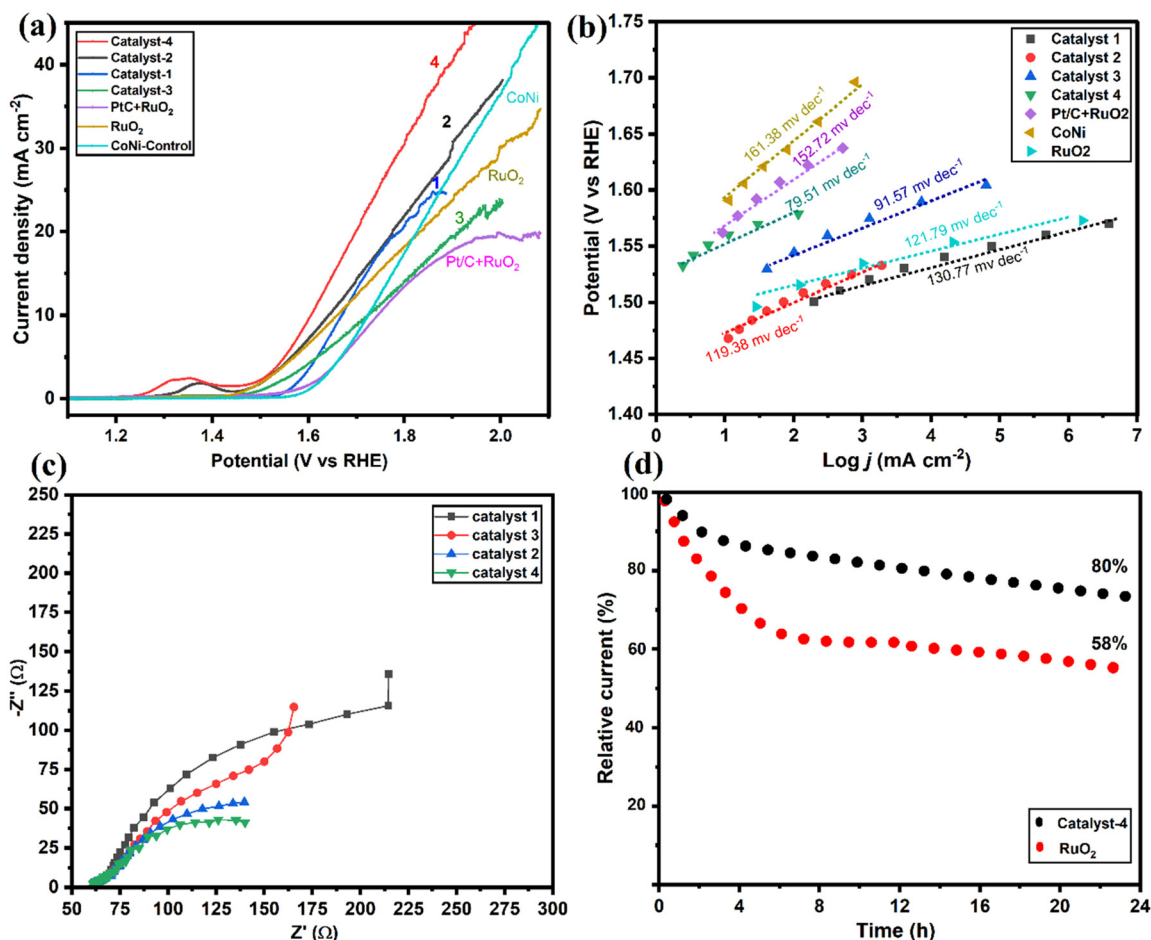
Fig. 7 Electrochemical OER performances: (a) LSV curves of CoS/Co-N x /CoNi/NiS 2 @CNS-1–4, commercial RuO 2 and Pt/C + RuO 2 in N 2 -saturated 0.1 M KOH, (b) Tafel plots of LSV curves of catalysts 1–4, RuO 2 and Pt/C + RuO 2 , (c) EIS spectra of catalysts 1–4, and (d) chronoamperometric responses of Co 9 S 8 /Co-N/CoNi/Ni 3 S 2 @CNS-4, and commercial RuO 2 in N 2 -saturated 0.1 M KOH solution.
