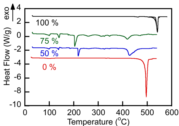
Fig. 3 DSC melting endotherms on 10\text{ }^\circ\text{C min}^{-1} heating of the carbonate ( \text{Li}_{1.24}\text{K}_{0.76}\text{CO}_3 ) and borate ( \text{Li}_{1.5}\text{Na}_{1.5}\text{BO}_3 ) and their blends in nitrogen atmosphere. Numbers indicate nominal initial content of borate (mol%) in the blends. Endotherms were shifted along the heat flow axis for the presentation clarity, while preserving the original scale. Solid and dashed lines represent endotherms obtained using a Discovery DSC 250 (sealed pans) and Q600 (open to nitrogen atmosphere), respectively.
