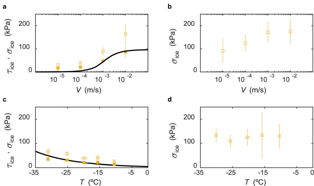
Fig. 5 Effect of mode of ice adhesion test. (a and b) Variation of \tau_{ice} (filled) and \sigma_{ice} (unfilled) with shear velocity, V , at surface temperature, T = -20\text{ }^{\circ}\text{C} , and elastomer thickness, h = 35\text{ }\mu\text{m} in mixed and normal mode tests, respectively. The black solid curve in (a) indicates 0.45\tau_{ice,s} where \tau_{ice,s} = \tau_{friction} (using eqn (1)) is the ice adhesion strength in the shear mode when all the other experimental conditions are the same. (c and d) Variation of \tau_{ice} (filled) and \sigma_{ice} (unfilled) with T , at V = 0.1\text{ mm s}^{-1} , and h = 35\text{ }\mu\text{m} in mixed and normal mode tests, respectively. The black solid curve in (c) indicates the Williams-Landel-Ferry transformation. Error bars represent standard deviation for n_e \geq 3 independent experiments.
