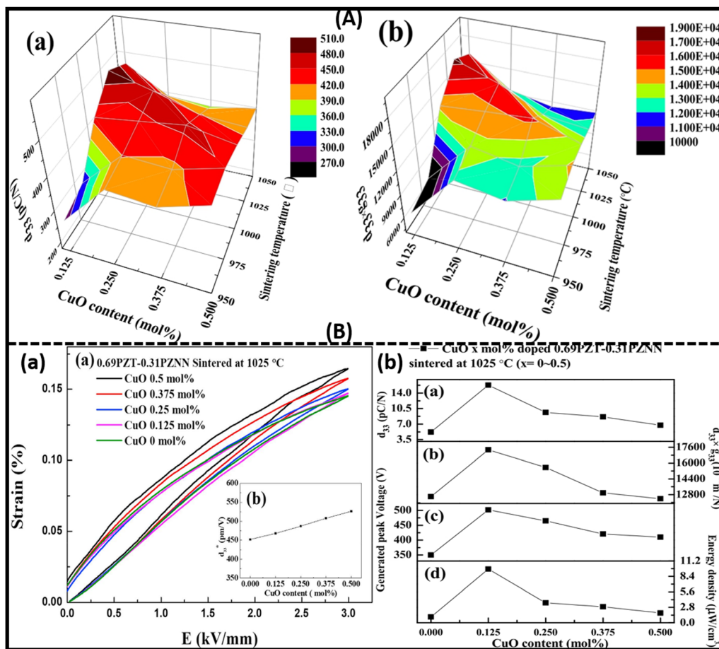
Fig. 22 (A) and (B) Fluctuation of the piezoelectric properties with respect to the sintering temperature and CuO dopant percentage in PNN–PZT using a 3D model, S-E loop, and 2D plot. A(a and b) 3D plots of d_{33} and d_{33} \times g_{33} with CuO content and sintering temperature. B(a) Deviation of the S-E loop with CuO proportion in the PNN–PZT composite; and (b) variation of the voltage output, d_{33} , d_{33} \times g_{33} , and energy density with CuO doping; reproduced with permission from ref. 307. Copyright Elsevier publications.
