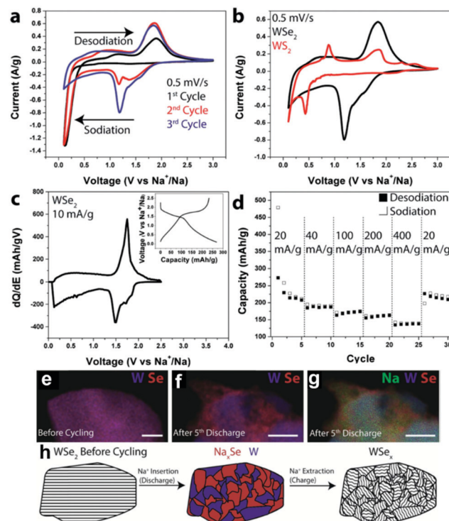
Fig. 12 (a) CV scans for the first three cycles from WSe 2 devices with CMC and EC/DEC. (b) CV scans comparing the energetics of chemical storage in WSe 2 and WS 2 during the 3rd cycle. (c) dQ/dE of a WSe 2 electrode at 10 mA g -1 ; inset: charge–discharge curves at 10 mA g -1 . (d) Galvanostatic rate study at 20, 40, 100, 200, and 400 mA g -1 . (e) EDS composite map of a WSe 2 electrode before cycling; scale bar \frac{1}{4} 100 nm. (f) EDS composite map of a WSe 2 battery electrode after the 5th discharge showing W and Se; scale bar \frac{1}{4} 100 nm. (g) The same EDS spectrum as (f) but with Na added. (h) Schematic illustrating the storage mechanism of Na in WSe 2 . Upon Na + insertion, segregated domains of Na 2 Se and W form. After Na + has been removed, WSe 2 is reformed, but it is less crystalline than in its original state. (Figure reproduced with permission from RSC Advances, ref. 164.)
