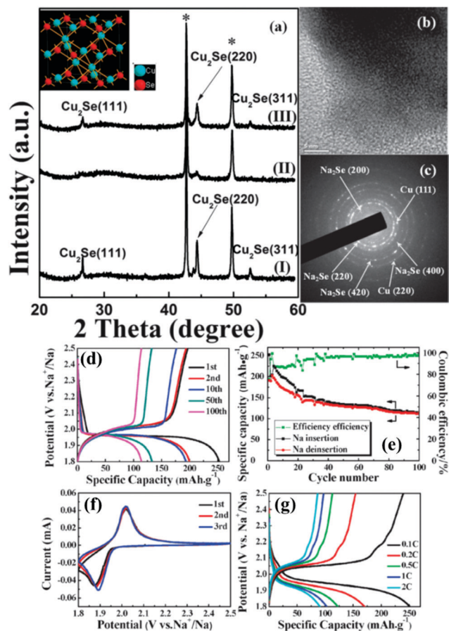
Fig. 11 (a) Ex situ XRD pattern of the Cu 2 Se thin film at various states during the first cycle of the Cu 2 Se/Na cell with a voltage range of 1.8–2.5 V. (I) As-prepared; (II) after discharging to 1.8 V; and (III) after charging to 2.5 V. The crystal structure of Cu 2 Se is shown in the inset. (b) TEM image and (c) corresponding SAED pattern after discharging to 1.8 V; (d) typical charge–discharge voltage profiles of the initial 100 cycles of the Na/NaClO 4 /Cu 2 Se battery at a constant current rate of 0.1 C between 1.8 and 2.5 V; (e) cycling performance of the Na/NaClO 4 /Cu 2 Se battery cycled at 0.1 C between 1.8 and 2.5 V; (f) the initial three CV curves of the Na/NaClO 4 /Cu 2 Se cell between 1.8 V and 2.5 V versus Na + /Na at a scan rate of 0.1 mV s -1 ; (g) charge–discharge curves at various current densities (0.1 C, 0.2 C, 0.5 C, 1 C, and 2 C). (Figure reproduced with permission from Chem Comm. (RSC), ref. 163.)
