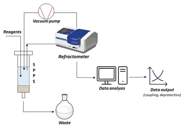
Fig. 8 Schematic representation of SPPS real-time monitoring by refractive index.
