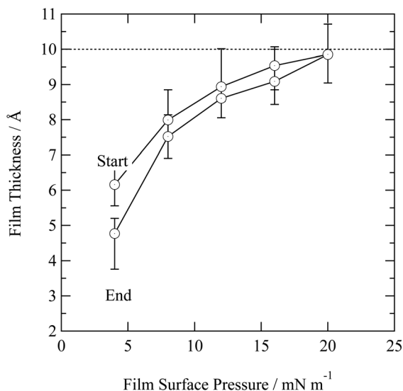
Fig. 4 Film thickness as a function of film surface pressure for the urban aerosol extract. The uncertainty in film thickness was estimated from fitting neutron reflectivity profiles. Surface pressure greater than 20 \text{ mN m}^{-1} were not recorded owing to limited sample. The dashed horizontal line represents a film thickness of 10 \text{ Å} and may be indicative of a typical compressed film thickness.
