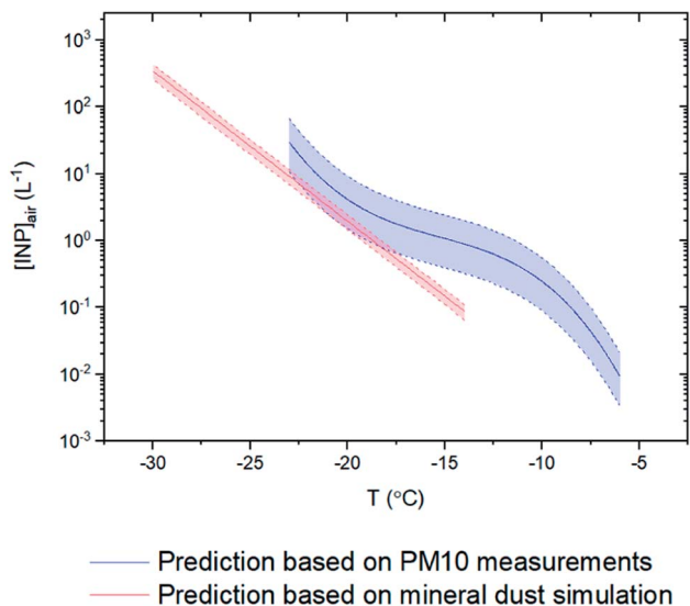
Fig. 9 Prediction curves for the average numbers of INPs per volume of air ( [\text{INP}]_{\text{air}} ) from May 10 th to May 29 th 2018. The blue curve corresponds to predictions using measured PM10 concentrations at the site (Fig. 8) and the n_m parameterization for the glacier dust samples determined here (Fig. 5). The red curve corresponds to predictions using simulated surface areas of natural mineral dust at the site from low latitude sources using GEOS-Chem and an n_s parameterization from Ullrich et al. 52 Error bars are based on the 95% confidence level of mineral dust mass/surface area from the filters/simulations from May 10 th to May 29 th and the 95% confidence level in the n_m parameterization for the glacier dust samples.
